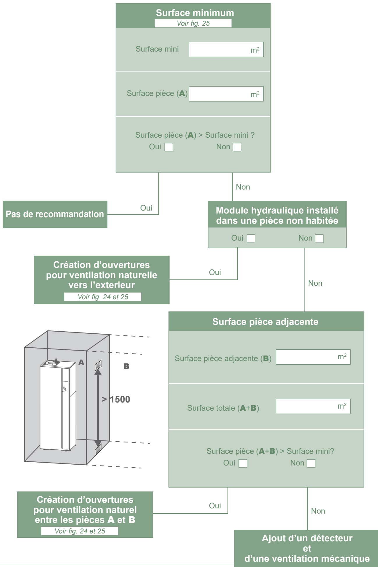
fig. 27 - Surface minimale
